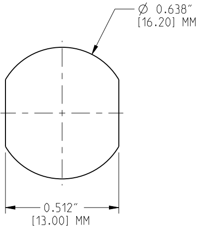
RECOMMENDED MOUNTING HOLE DIMENSIONS
